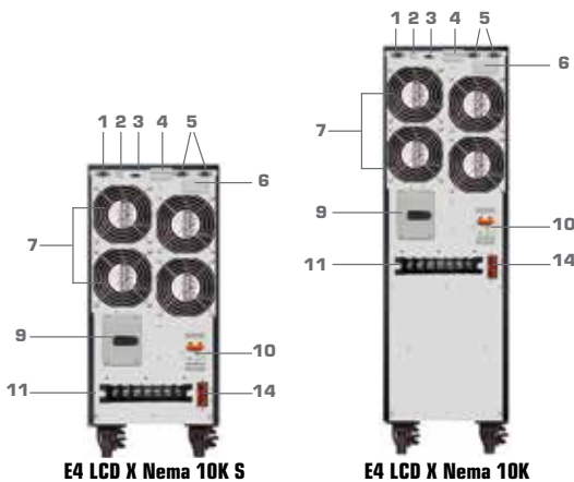
E4 LCD X Nema 10K S
